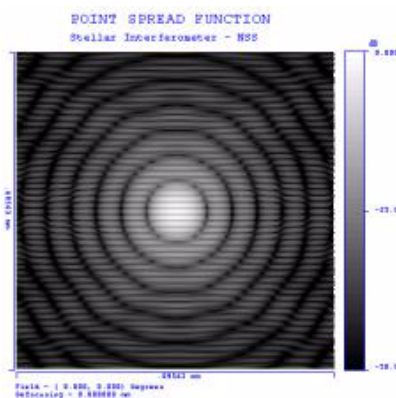
Figure 10b. PSF for Aligned System
