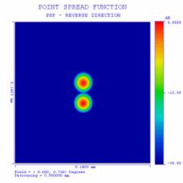
Figure 8c. Field Intensity at Input Fiber from Reflection at Output Fiber
