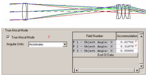
Figure 4. 5x40 Telescope & True Afocal Modeling Controls in CODE V
