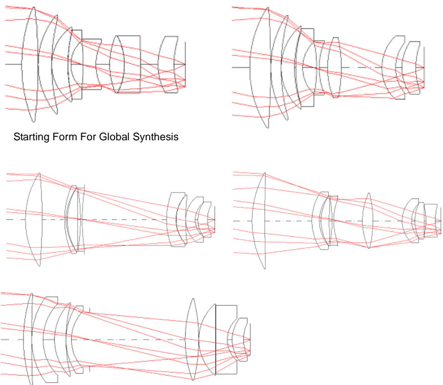
Figure 2. Several distinct solutions for a CRT camera lens, generated by Global Synthesis
