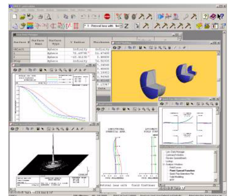
Figure 3. Several Analyses for a Petzval Lens
