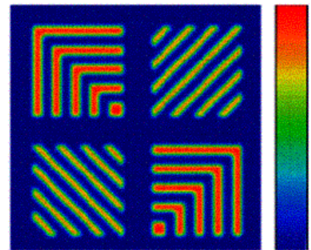
Figure 13. Offner 1:1 Microlithographic Projection system & 2-D Partial Coherence Analysis
