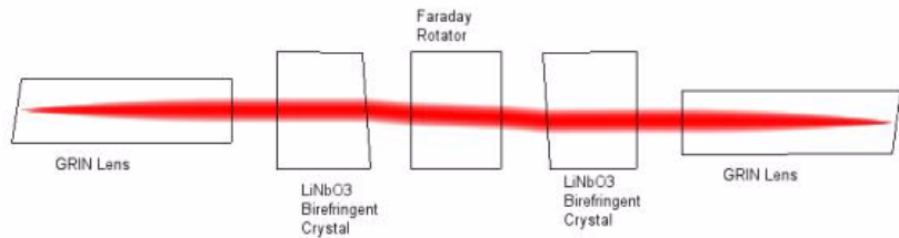
Figure 8a. Optical Isolator System
