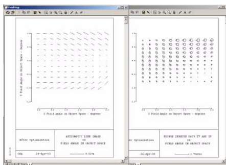
Figure 7. Full Field Maps of Aberration Fields
