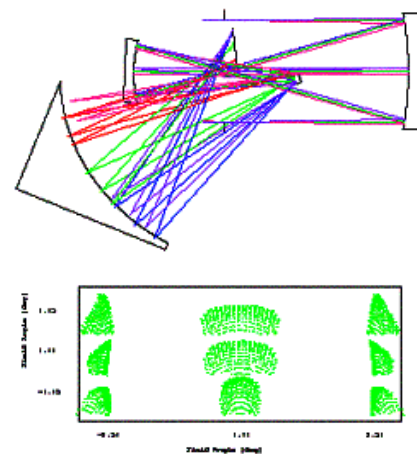
System Layout and Full Field Spot Diagram - Before Optimization
