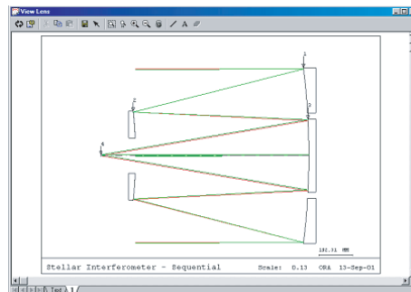
Figure 10a. Stellar Interferometer Systems
