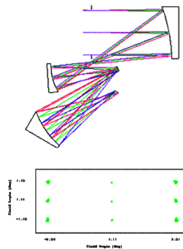
System Layout and Full Field Spot Diagram - After Optimization (same scale)
