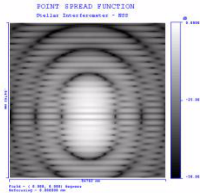
Figure 10c. PSF for Misaligned System
