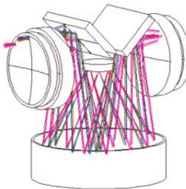
Figure 13. Offner 1:1 Microlithographic Projection system & 2-D Partial Coherence Analysis
